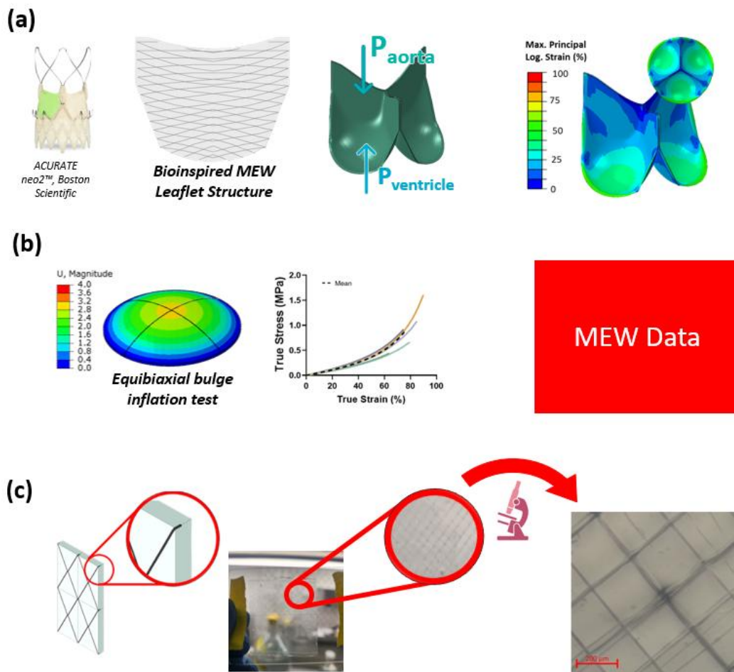
Figure 1: (a) Computational modelling of fibre-embedded polymer valve, (b) material calibration against bulge inflation tests of polymer material with and without fibre embedding, (c) structure of manufactured polymer composite compared to computational model
